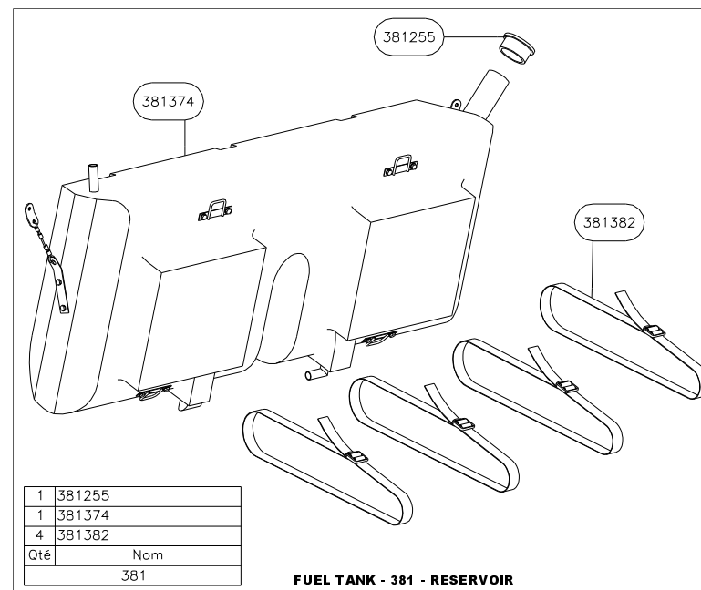
FUEL TANK - 381 - RESERVOIR
