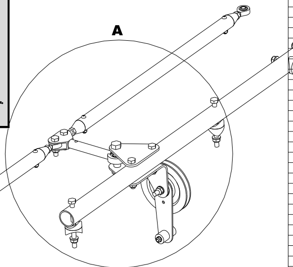
AILERON CABIN MECHANISM TOP - 352 - COMMANDE AILERON HAUT CABINE Type 3
