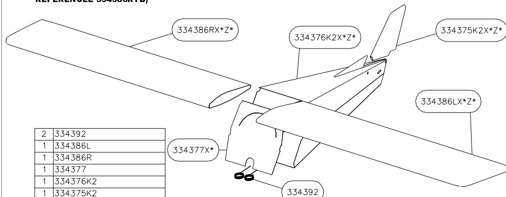
SAILS - 334 - TOILES Type 2
