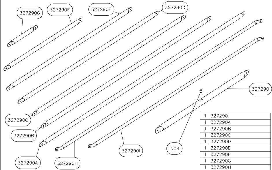
LONGITUDINAL FUSELAGE RIBS - 326 - TUBES DE FUSELAGE LONGITUTINAUX
