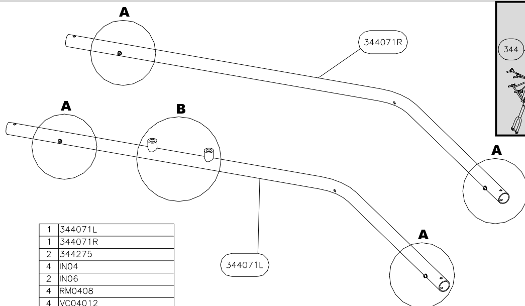
DOOR ENTRY TUBES BOTTOM - 344 - TUBES ENTREE DE CABINE INFERIEURS
