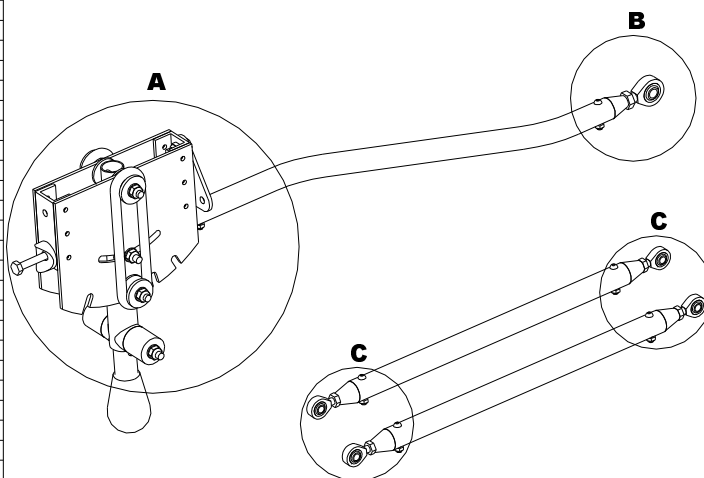
FLAP CONTROL - 368 - COMMANDE DE VOLETS Type 3
