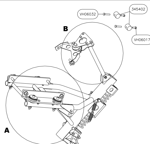
Rotax 912 ENGINE BRACKET - 345 - SUPPORT MOTEUR Rotax 912 Type 2
