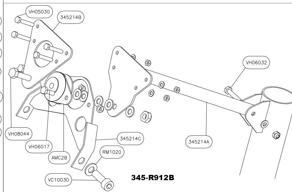
Rotax 912 ENGINE BRACKET - 345 - SUPPORT MOTEUR Rotax 912 Type 2
