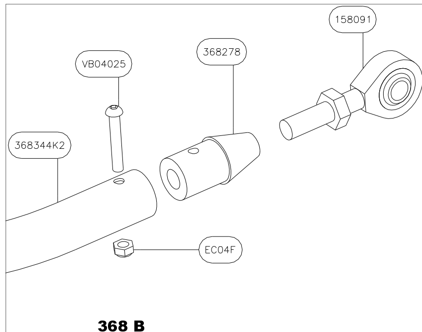
FLAP CONTROL - 368 - COMMANDE DE VOLETS Type 3
