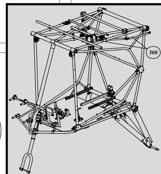
FLAP CONTROL - 368 - COMMANDE DE VOLETS Type 3
